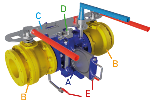
Double Block Bleed & Blind - D3B
