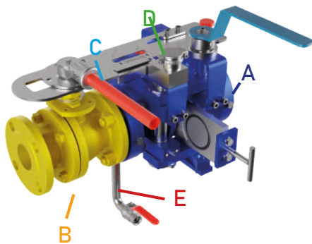
Single Block Bleed & Blind - S3B
